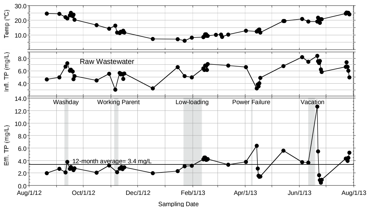
Figure 4-8. Influent and effluent total phosphorus (TP) concentrations and temperature versus time for the Woodchip Bed treatment unit during the 12-month verification testing period.
