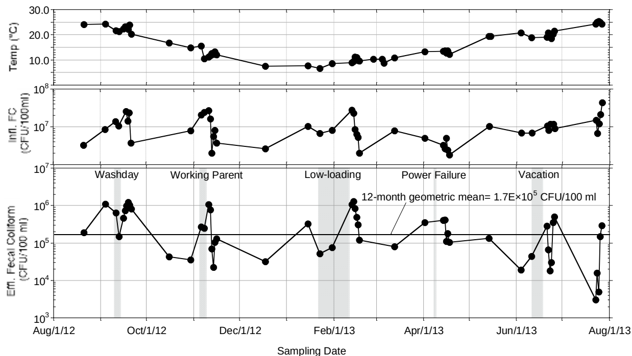
Figure 4-4. Influent and effluent fecal coliform (FC) concentrations and temperature versus time for the RGF treatment unit during the 12-month verification testing period.
