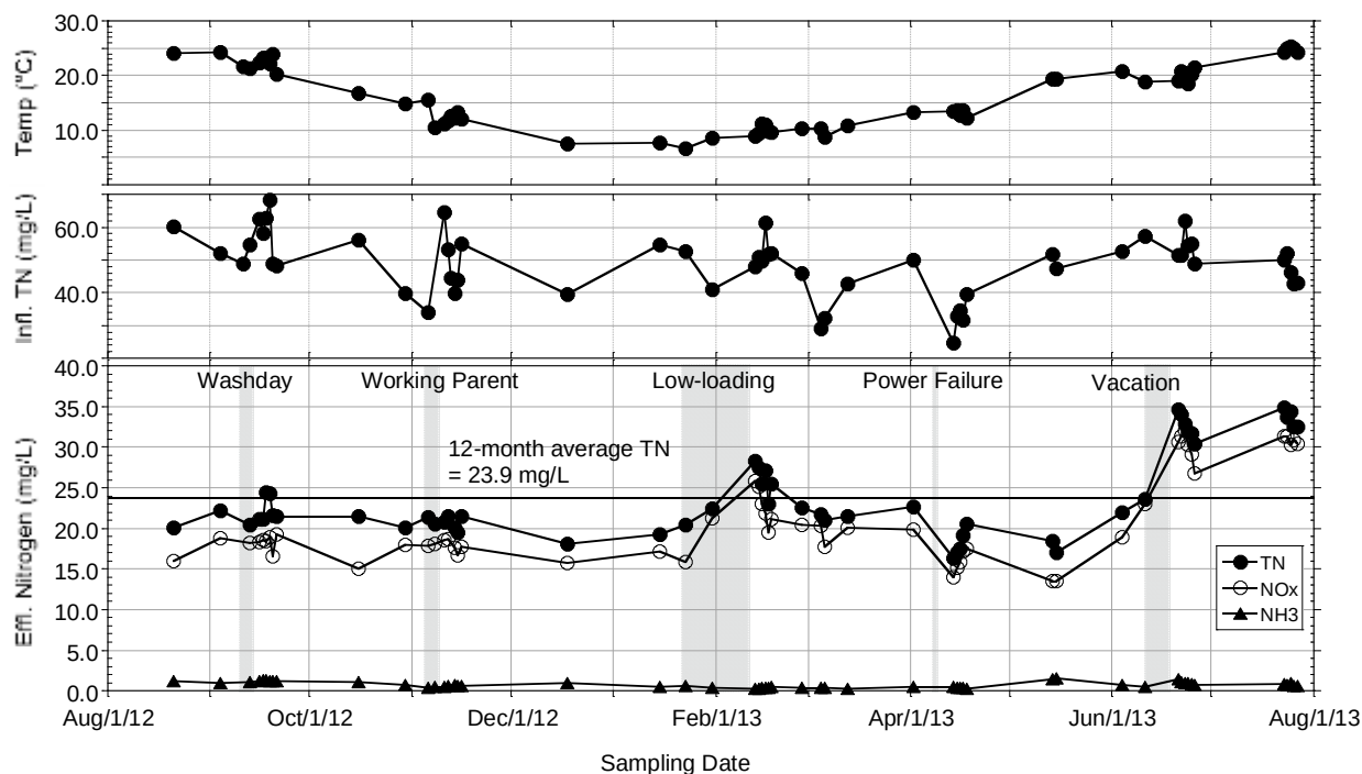
Figure 4-1. Influent TN and effluent TN, \text{NH}_3\text{-N} , and \text{NOx-N} concentrations and temperature versus time for the RGF treatment unit during the 12-month verification testing period.
