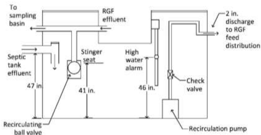
Figure 2-2. Recirculation basin for the Recirculating Gravel Filter.
